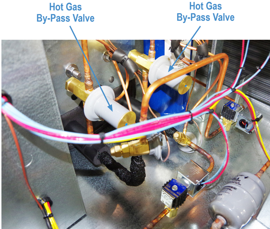
Hot Gas Bypass Valves - Installed
