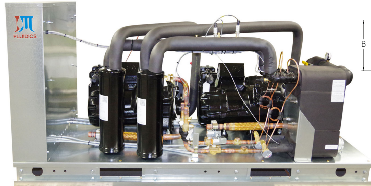
Indoor Chiller
