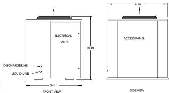
OC Refrigerant Connections: Discharge Line- 1/2", Liquid Line- 3/8"
