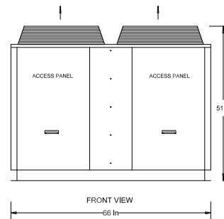
Outside Condenser Model (OC26D)
