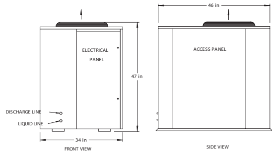
OC Refrigerant Connections: Discharge Line- 3/4", Liquid Line- 1/2"
