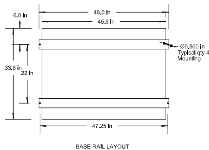
BASE RAIL LAYOUT
