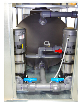
Inside View: Model: RRT600H, Dual Vertical 10 HP Process Pumps
