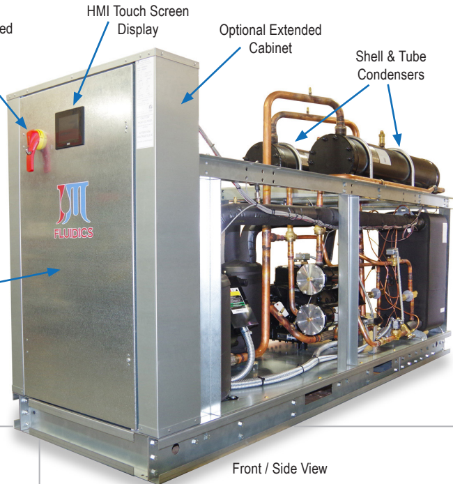
Electrical Cabinet
