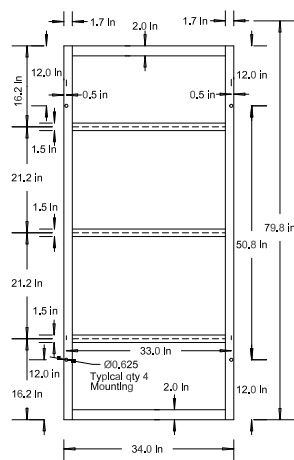
BASE FRAME LAYOUT
