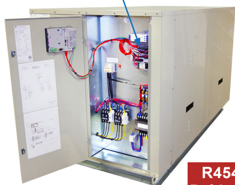
View Showing Electrical Panel Open
