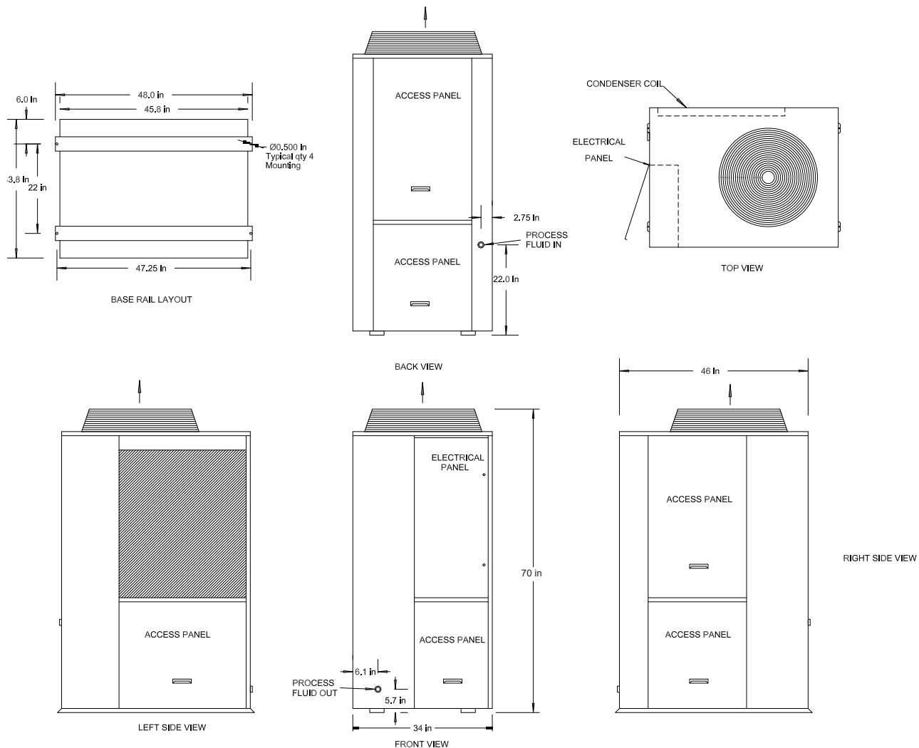
Dimensional & Electrical Table (Single Circuit)
